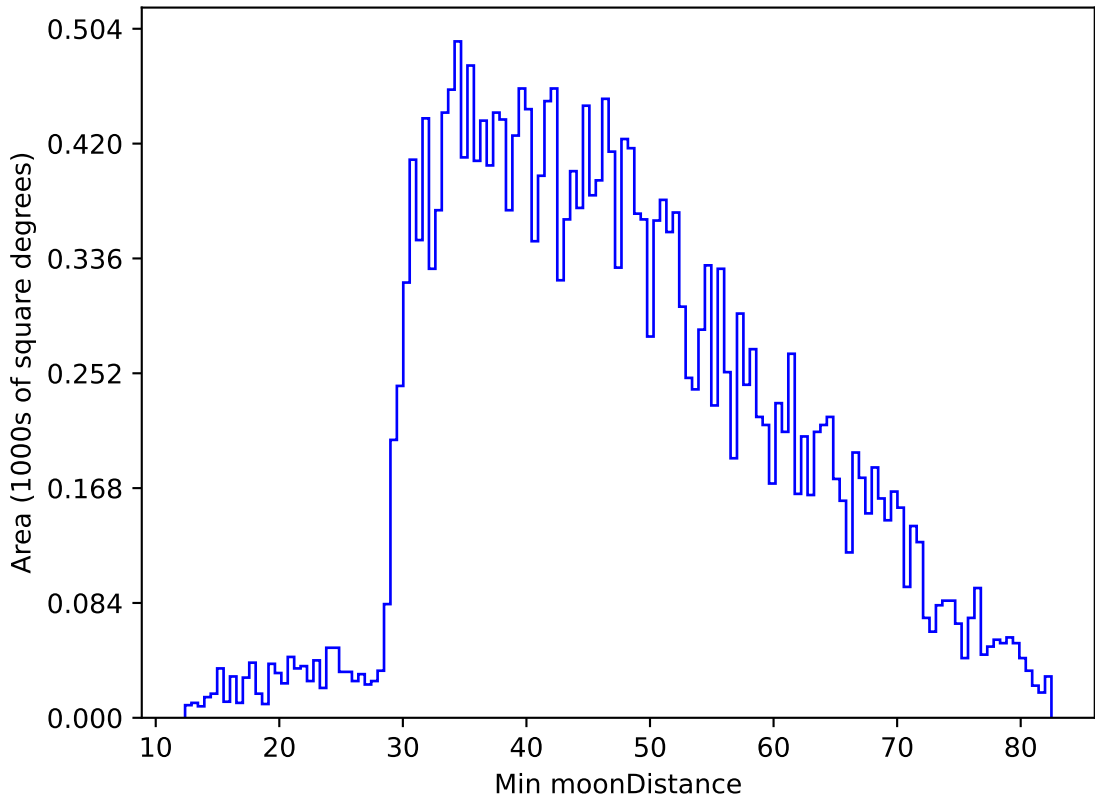
too_elab_r32_d2_griz_v3.4_10yrs All sky g band: Min moonDistance
