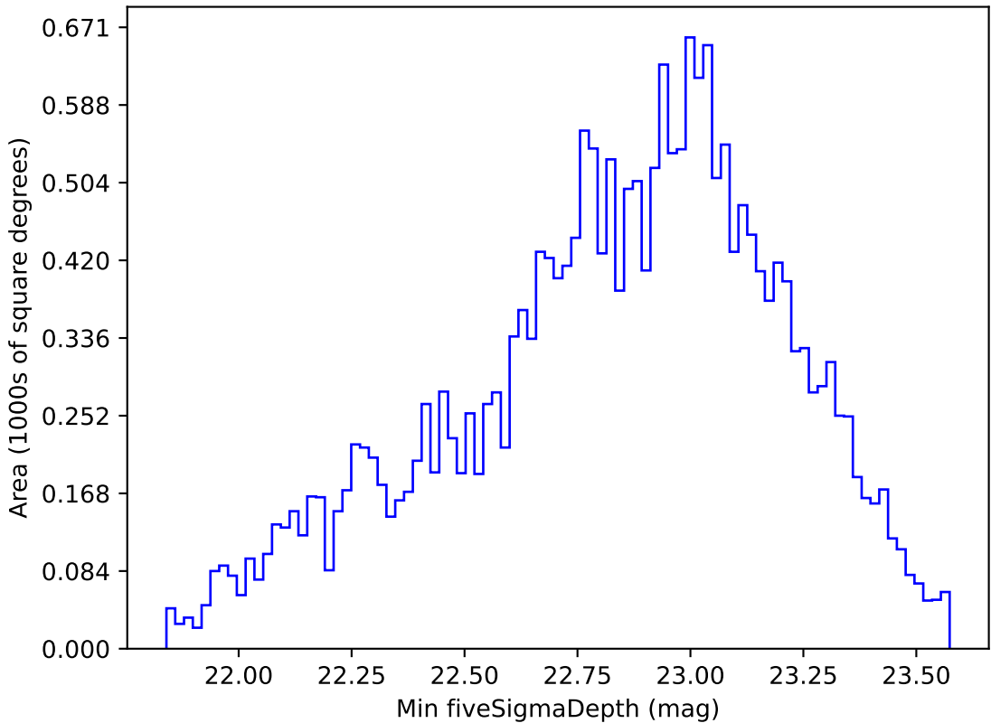
too_elab_r32_d2_griz_v3.4_10yrs Yr 1 u band: Min fiveSigmaDepth
