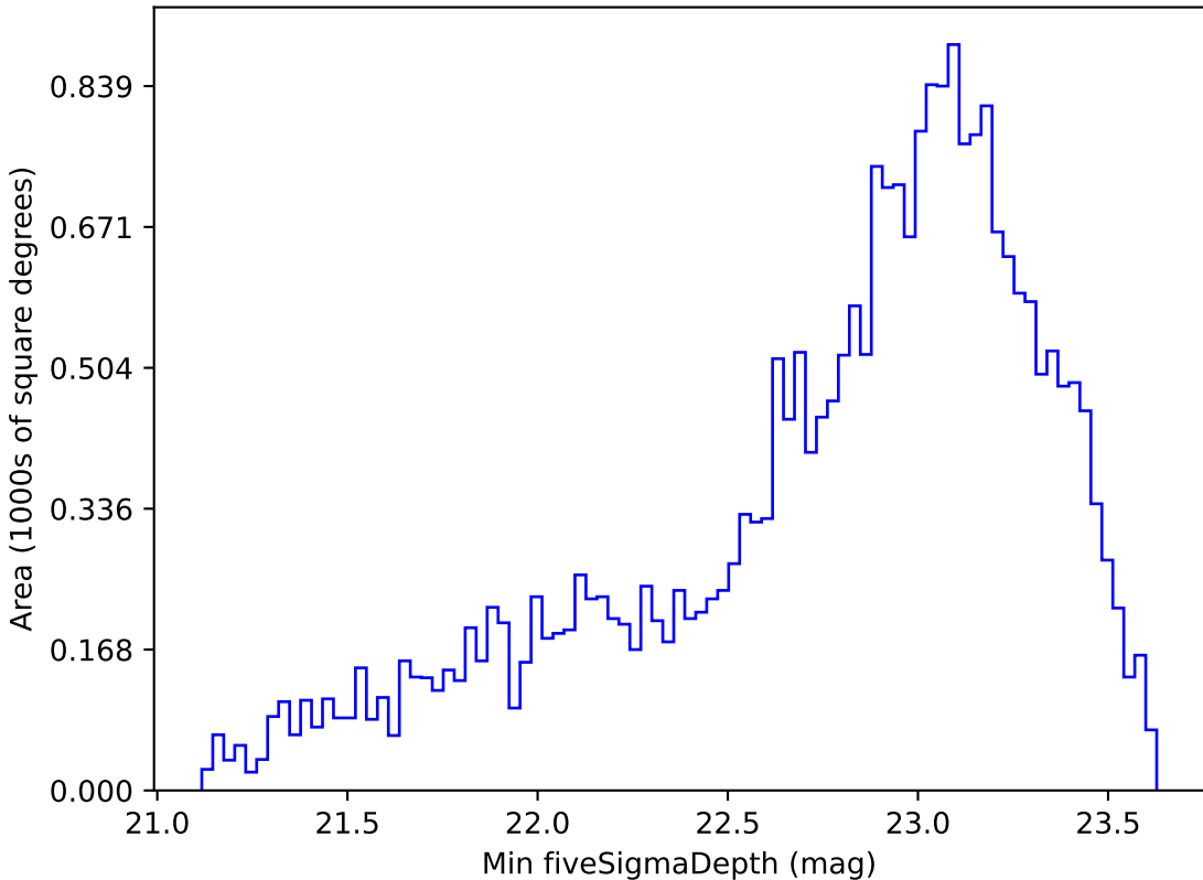
too_elab_r32_d2_griz_v3.4_10yrs Yr 1 i band: Min fiveSigmaDepth
