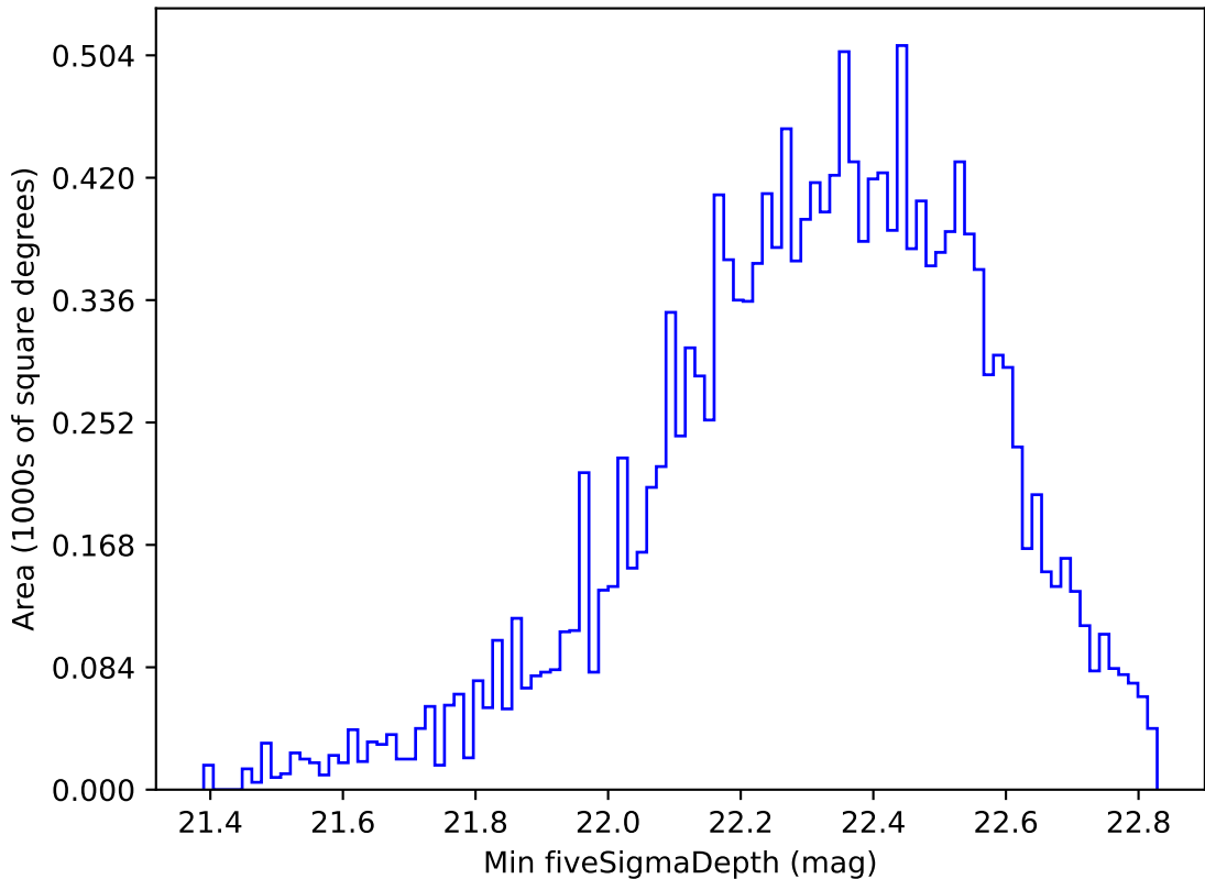
too_elab_r32_d2_griz_v3.4_10yrs WFD u band: Min fiveSigmaDepth
