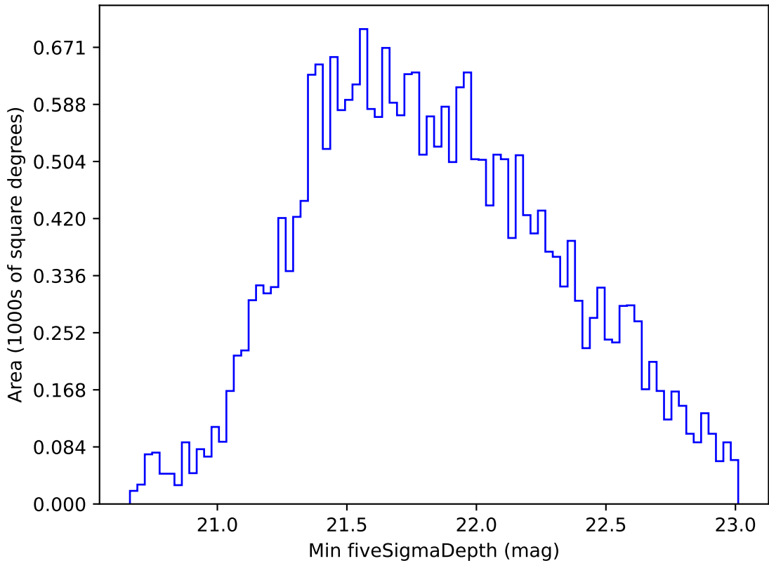
too_elab_r32_d2_griz_v3.4_10yrs All sky i band: Min fiveSigmaDepth
