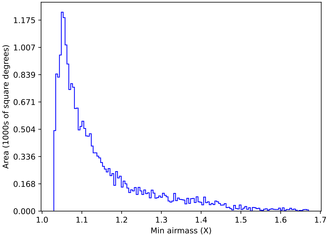
too_elab_r32_d2_griz_v3.4_10yrs Yr 1 u band: Min airmass
