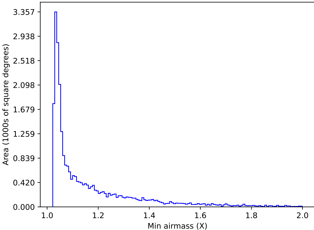
too_elab_r32_d2_griz_v3.4_10yrs Yr 1 i band: Min airmass
