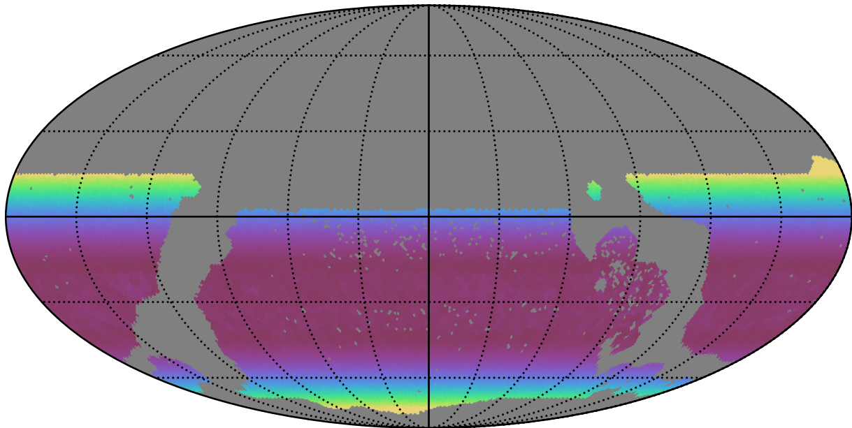
too_elab_r32_d2_griz_v3.4_10yrs WFD y band: Min airmass
