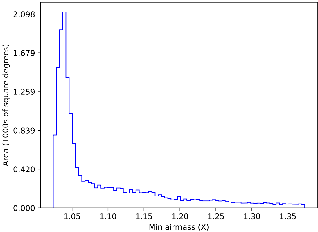
too_elab_r32_d2_griz_v3.4_10yrs WFD u band: Min airmass
