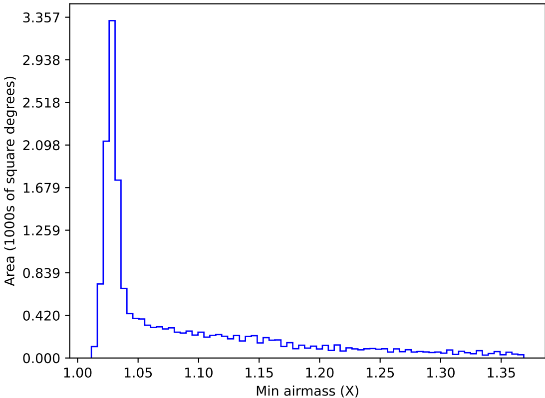
too_elab_r32_d2_griz_v3.4_10yrs WFD i band: Min airmass
