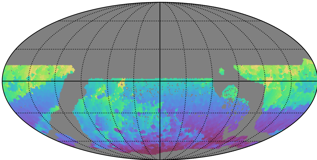
too_elab_r32_d2_griz_v3.4_10yrs WFD r band: Min HA
