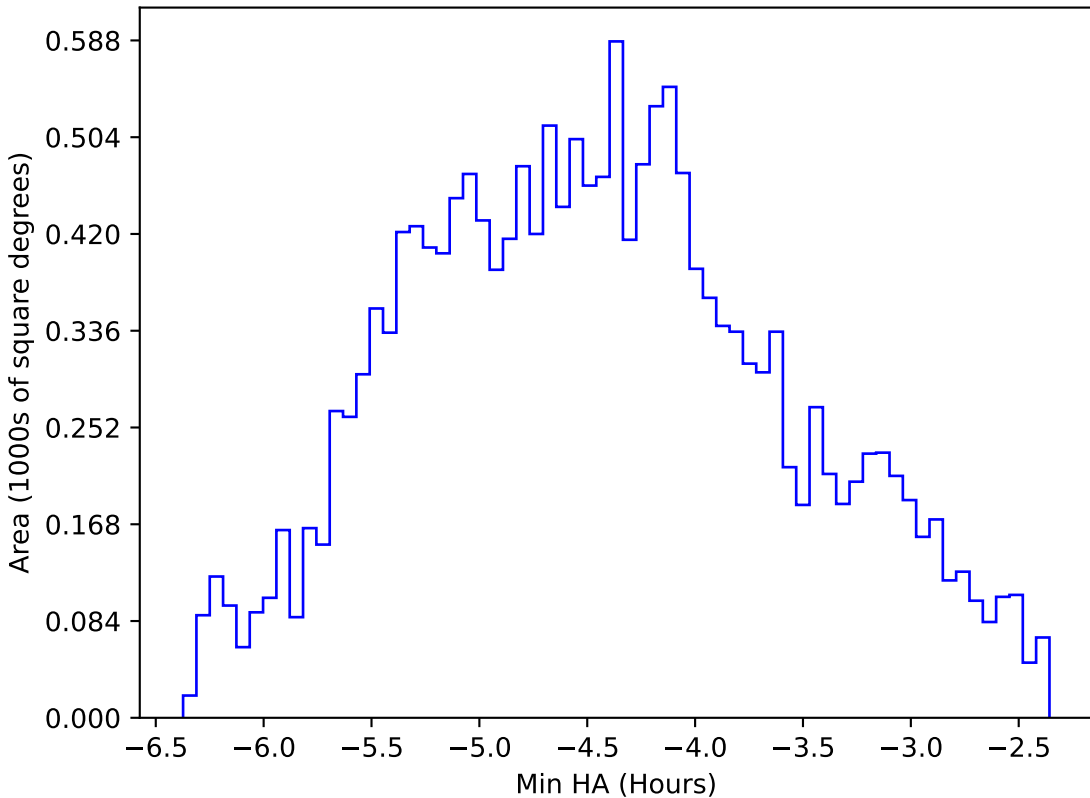
too_elab_r32_d2_griz_v3.4_10yrs WFD r band: Min HA
