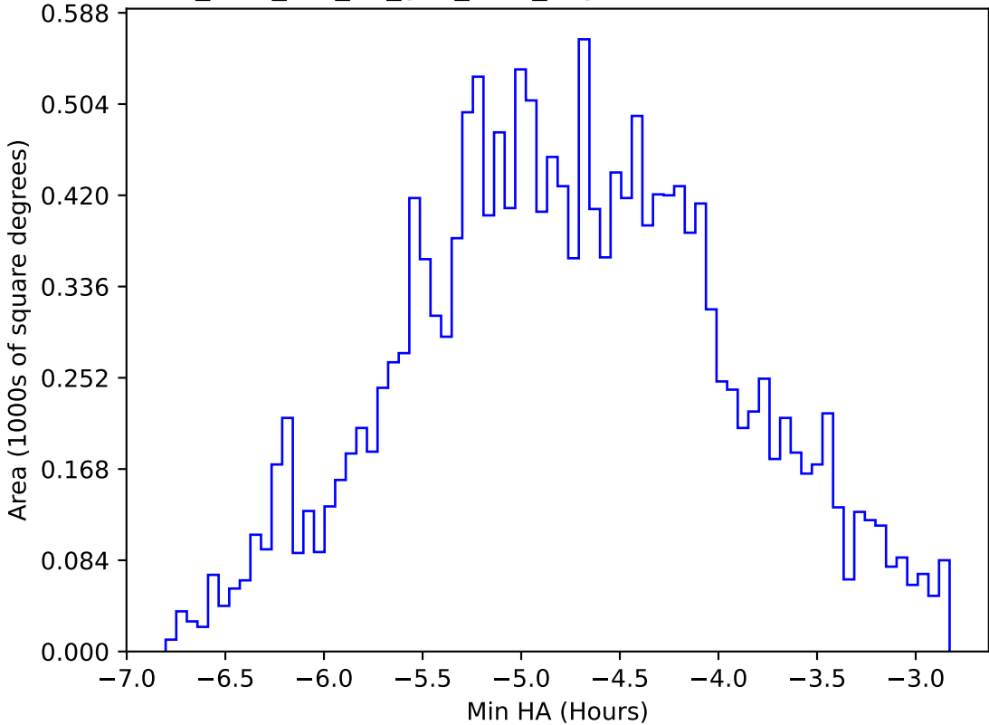
too_elab_r32_d2_griz_v3.4_10yrs WFD all bands: Min HA
