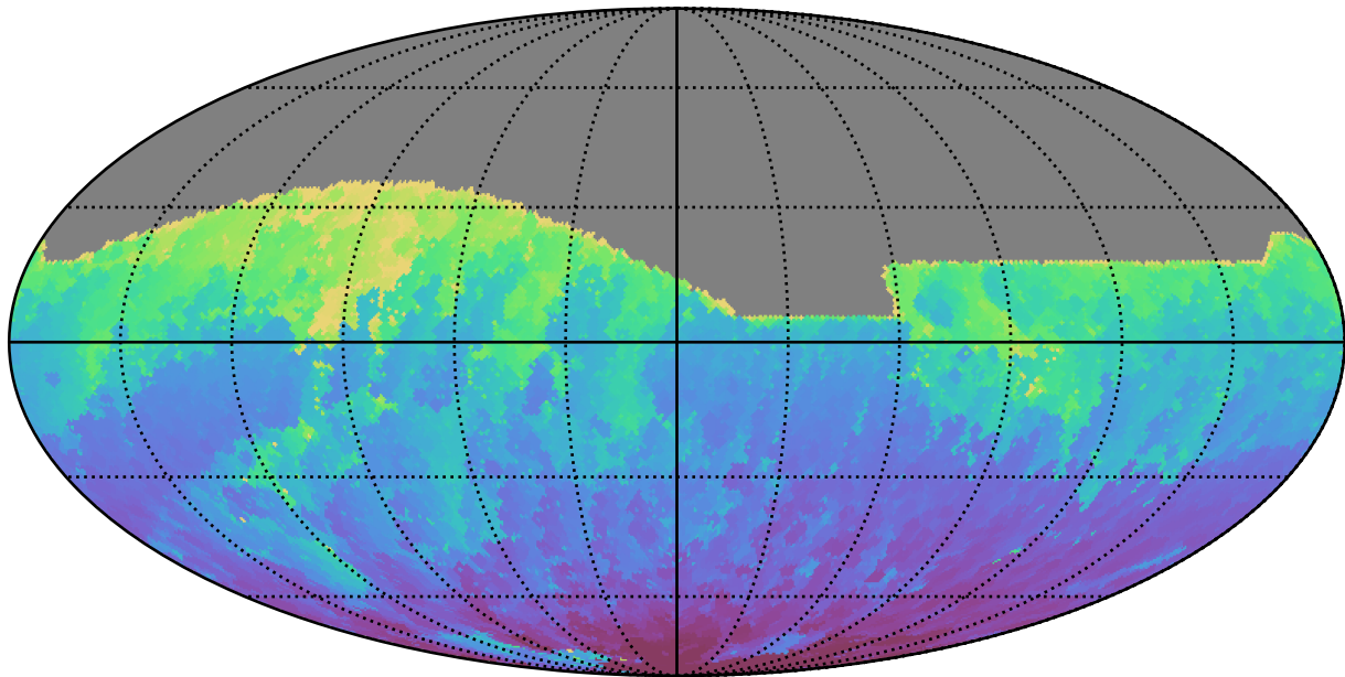
too_elab_r32_d2_griz_v3.4_10yrs All sky z band: Min HA
