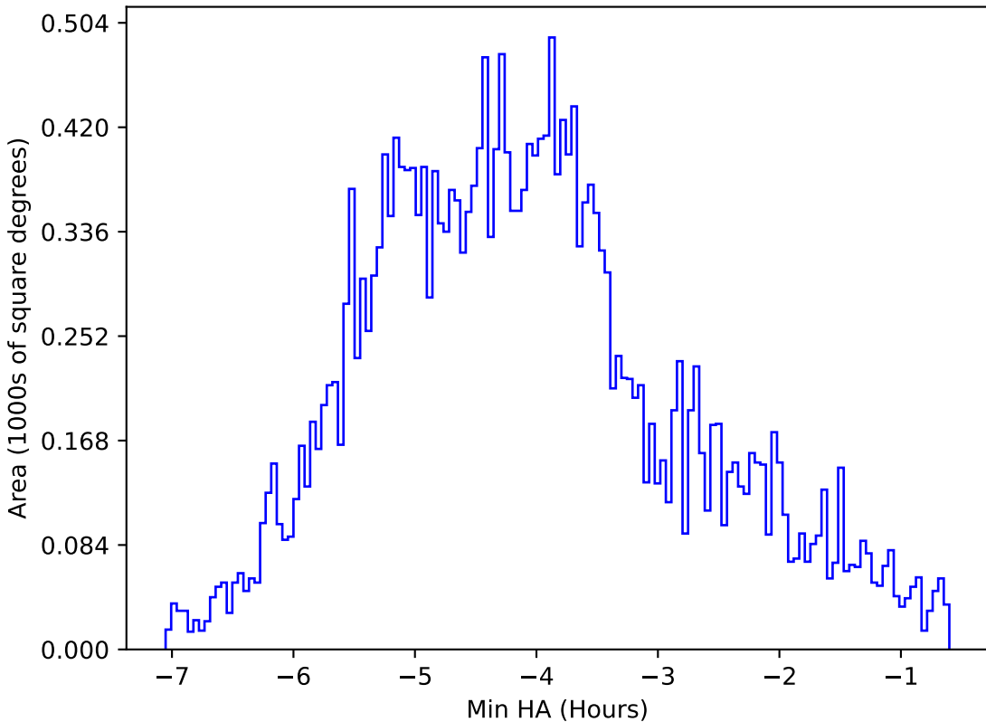
too_elab_r32_d2_griz_v3.4_10yrs All sky z band: Min HA
