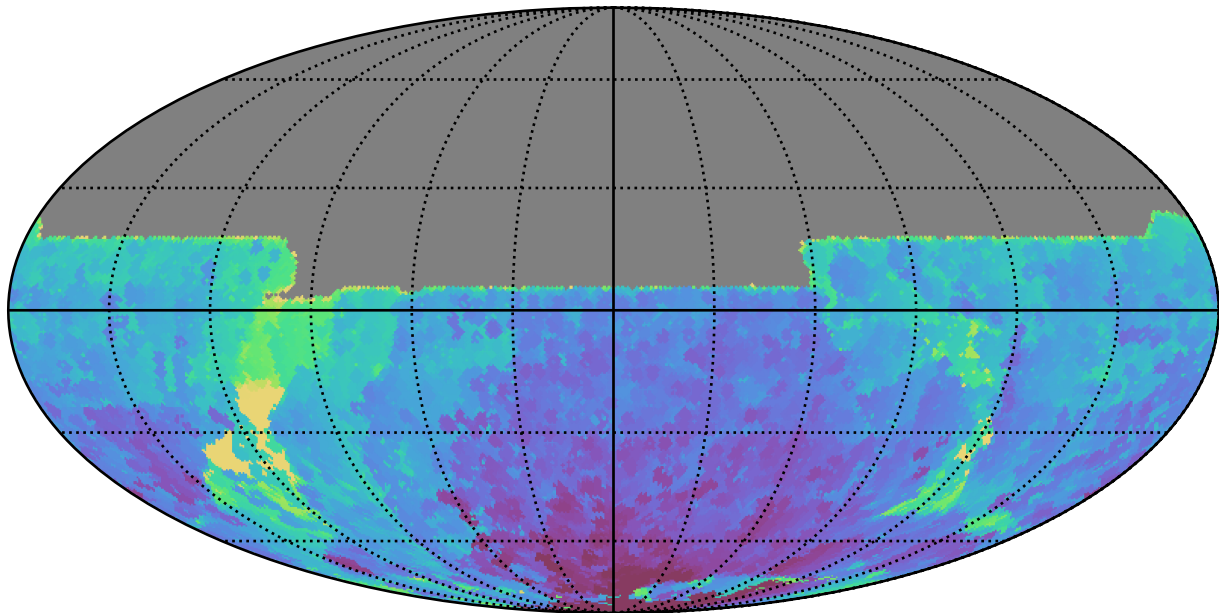
too_elab_r32_d2_griz_v3.4_10yrs All sky y band: Min HA
