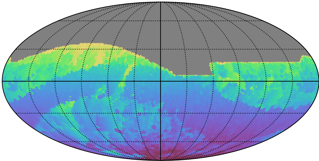
too_elab_r32_d2_griz_v3.4_10yrs All sky r band: Min HA
