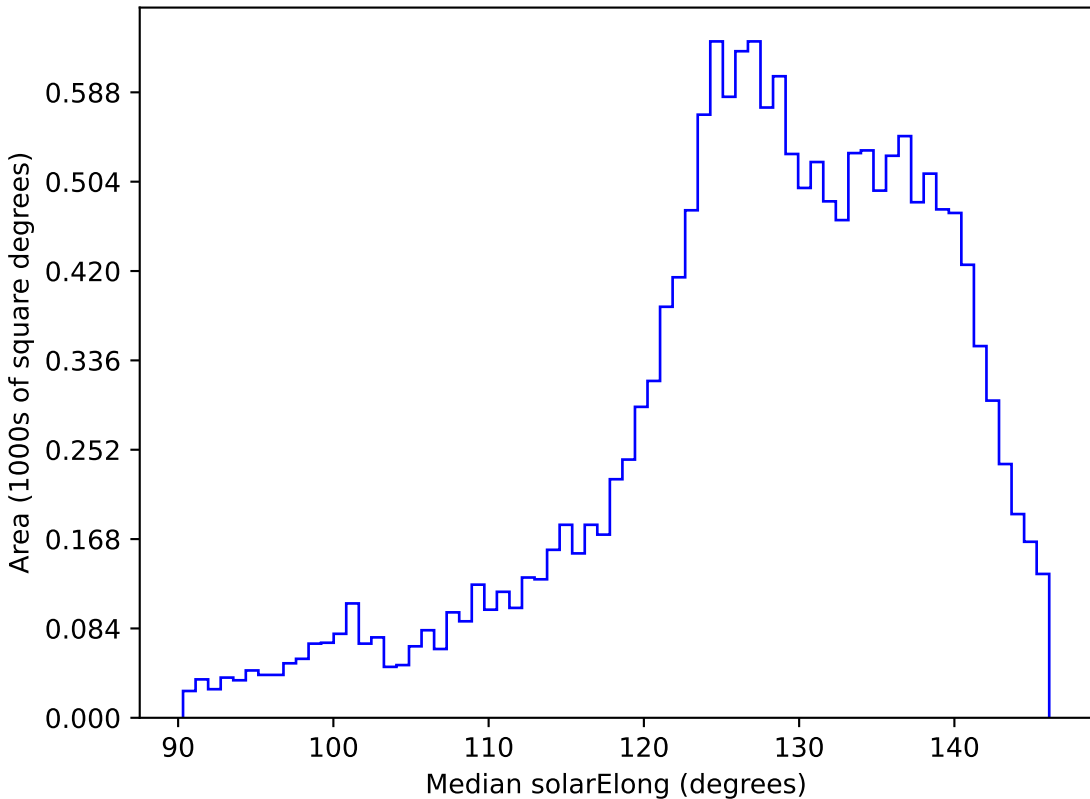
too_elab_r32_d2_griz_v3.4_10yrs WFD z band: Median solarElong
