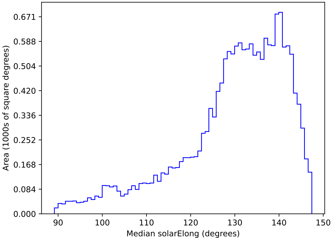
too_elab_r32_d2_griz_v3.4_10yrs WFD y band: Median solarElong
