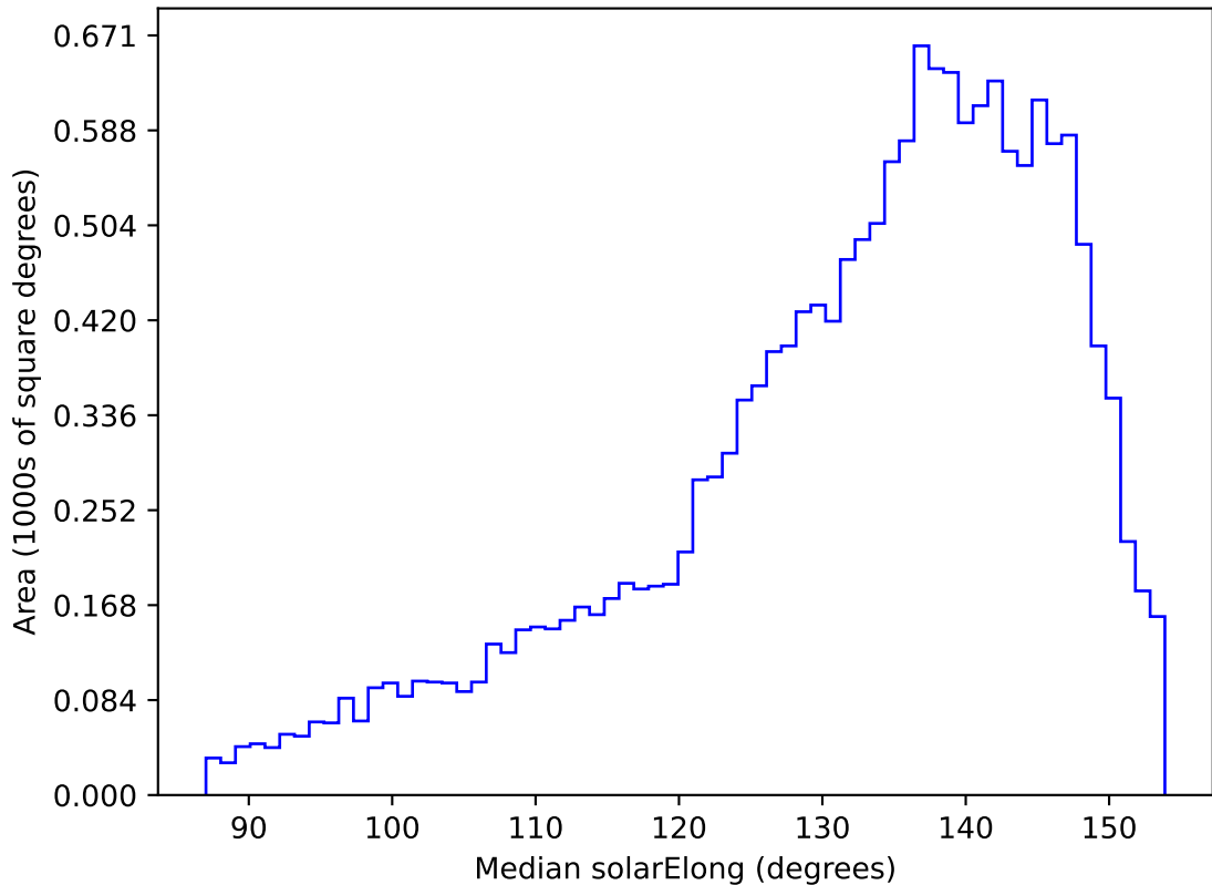
too_elab_r32_d2_griz_v3.4_10yrs WFD u band: Median solarElong
