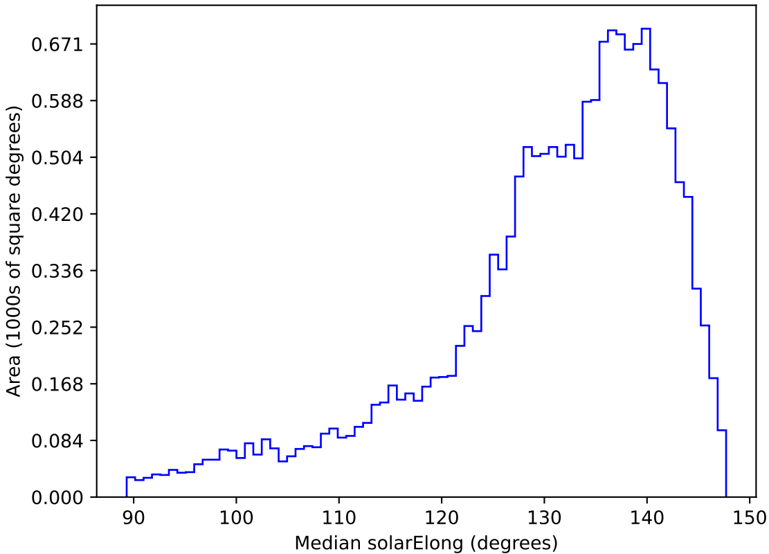
too_elab_r32_d2_griz_v3.4_10yrs WFD r band: Median solarElong
