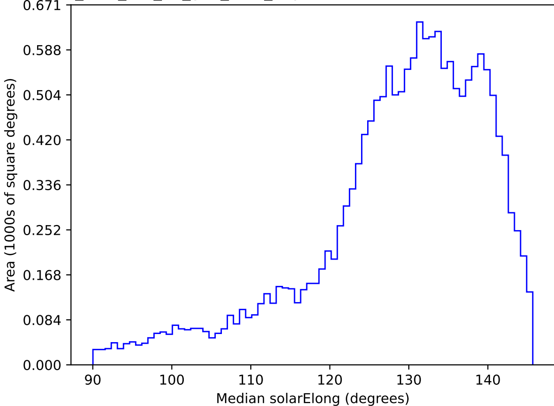
too_elab_r32_d2_griz_v3.4_10yrs WFD i band: Median solarElong
