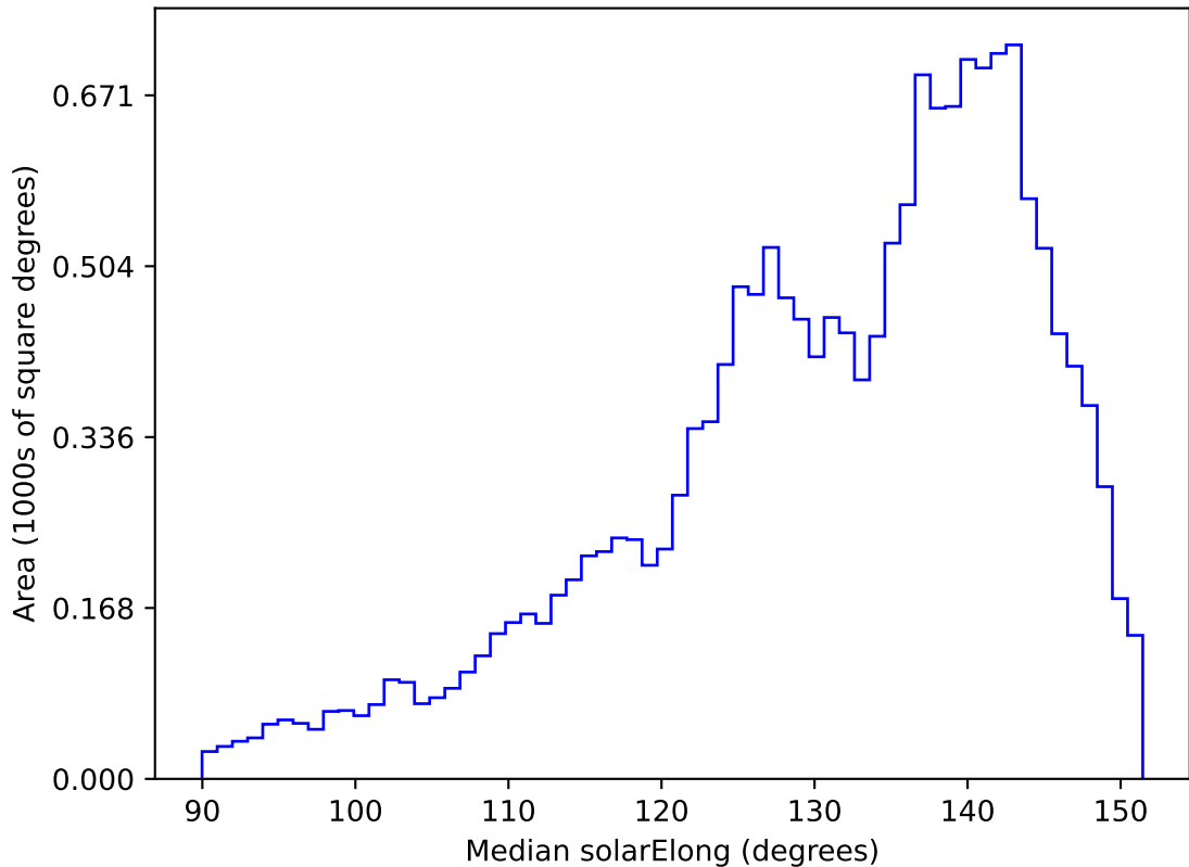
too_elab_r32_d2_griz_v3.4_10yrs WFD g band: Median solarElong
