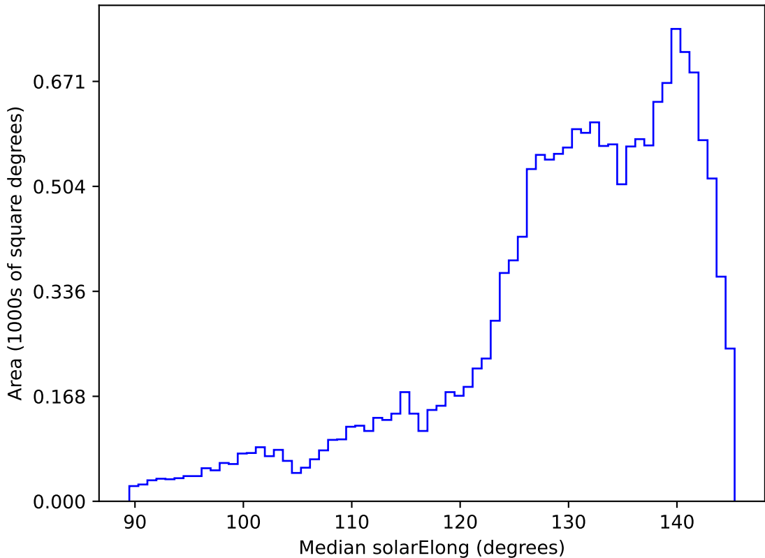
too_elab_r32_d2_griz_v3.4_10yrs WFD all bands: Median solarElong
