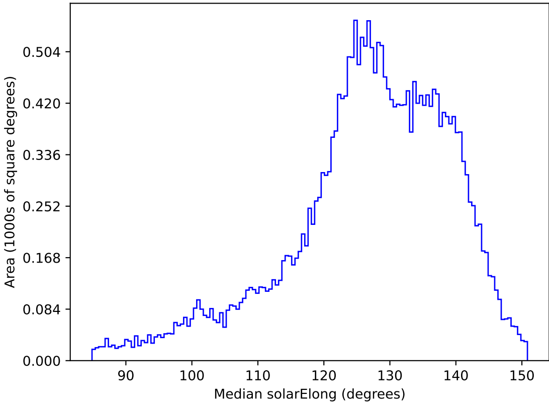
too_elab_r32_d2_griz_v3.4_10yrs All sky z band: Median solarElong
