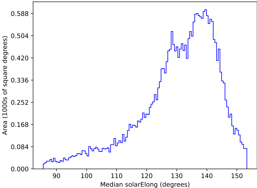
too_elab_r32_d2_griz_v3.4_10yrs All sky r band: Median solarElong
