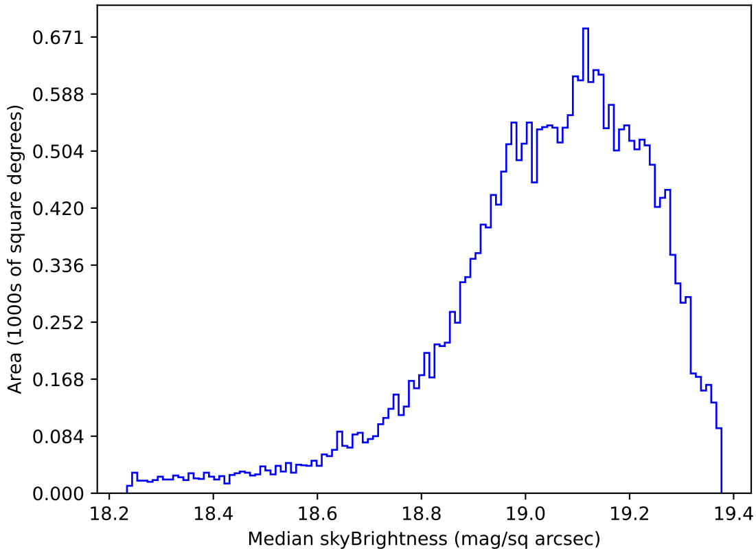
too_elab_r32_d2_griz_v3.4_10yrs Yr 1 z band: Median skyBrightness
