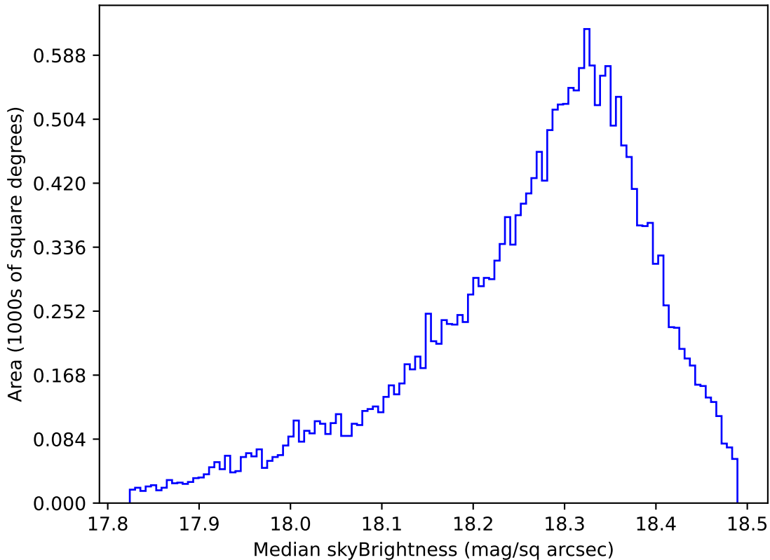
too_elab_r32_d2_griz_v3.4_10yrs Yr 1 y band: Median skyBrightness
