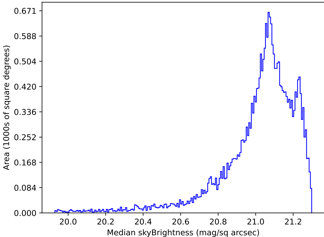
too_elab_r32_d2_griz_v3.4_10yrs Yr 1 r band: Median skyBrightness
