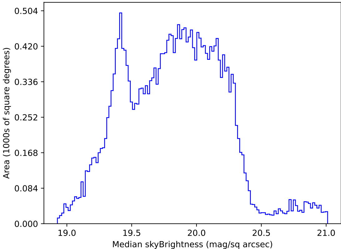
too_elab_r32_d2_griz_v3.4_10yrs Yr 1 all bands: Median skyBrightness
