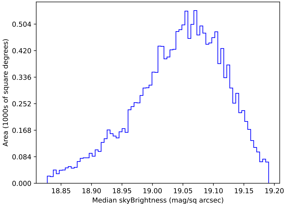
too_elab_r32_d2_griz_v3.4_10yrs WFD z band: Median skyBrightness
