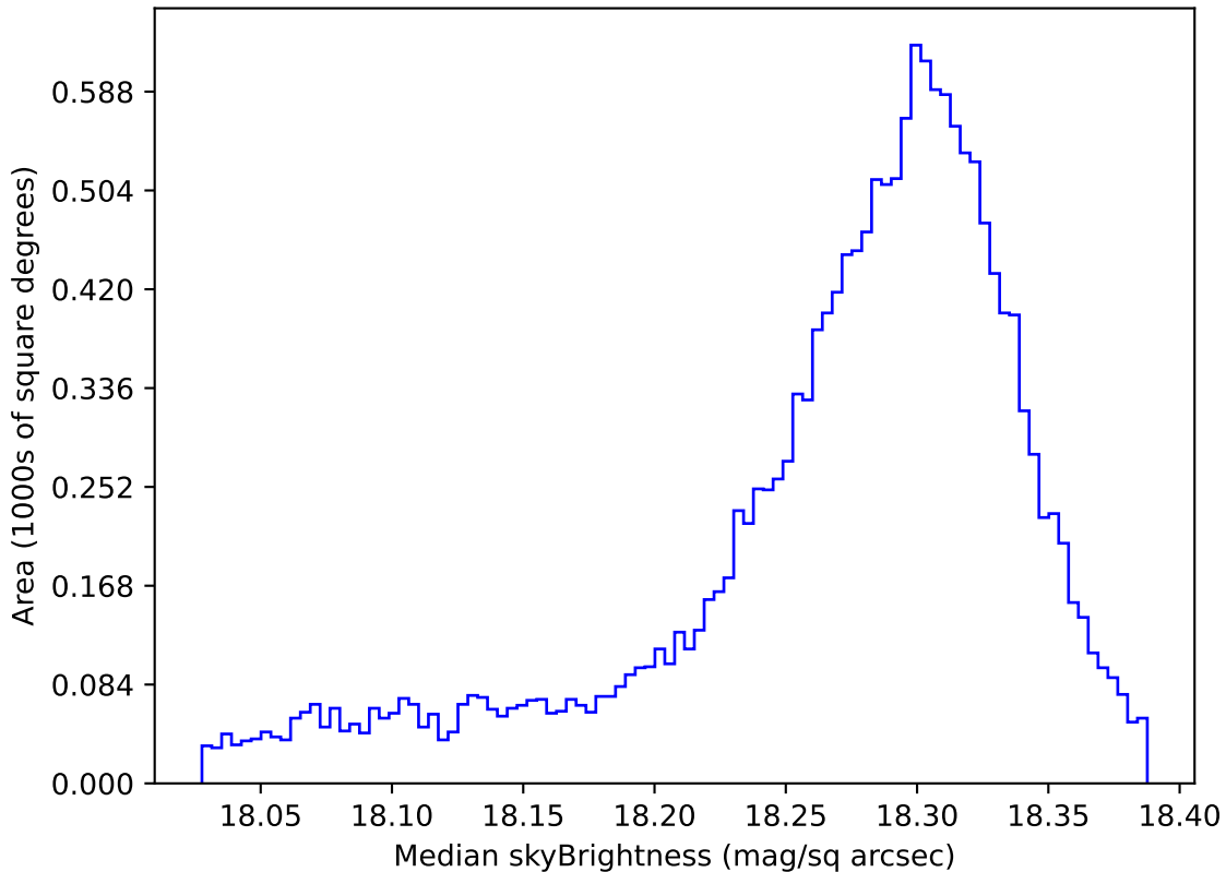
too_elab_r32_d2_griz_v3.4_10yrs WFD y band: Median skyBrightness
