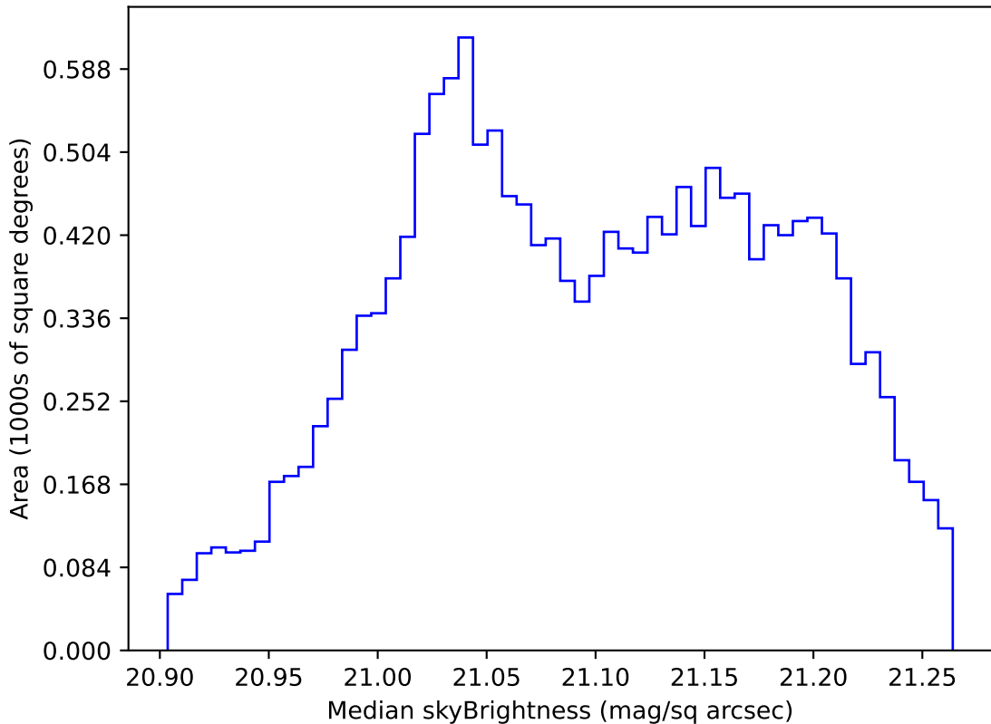
too_elab_r32_d2_griz_v3.4_10yrs WFD r band: Median skyBrightness
