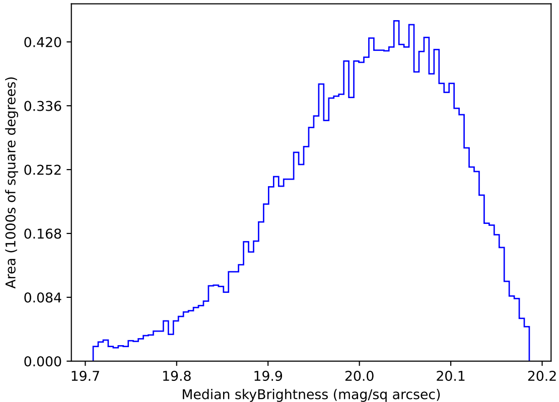
too_elab_r32_d2_griz_v3.4_10yrs WFD i band: Median skyBrightness
