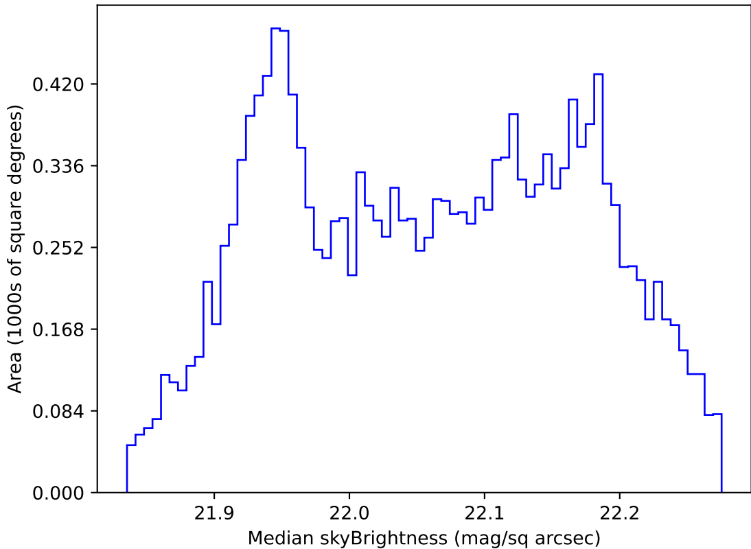
too_elab_r32_d2_griz_v3.4_10yrs WFD g band: Median skyBrightness
