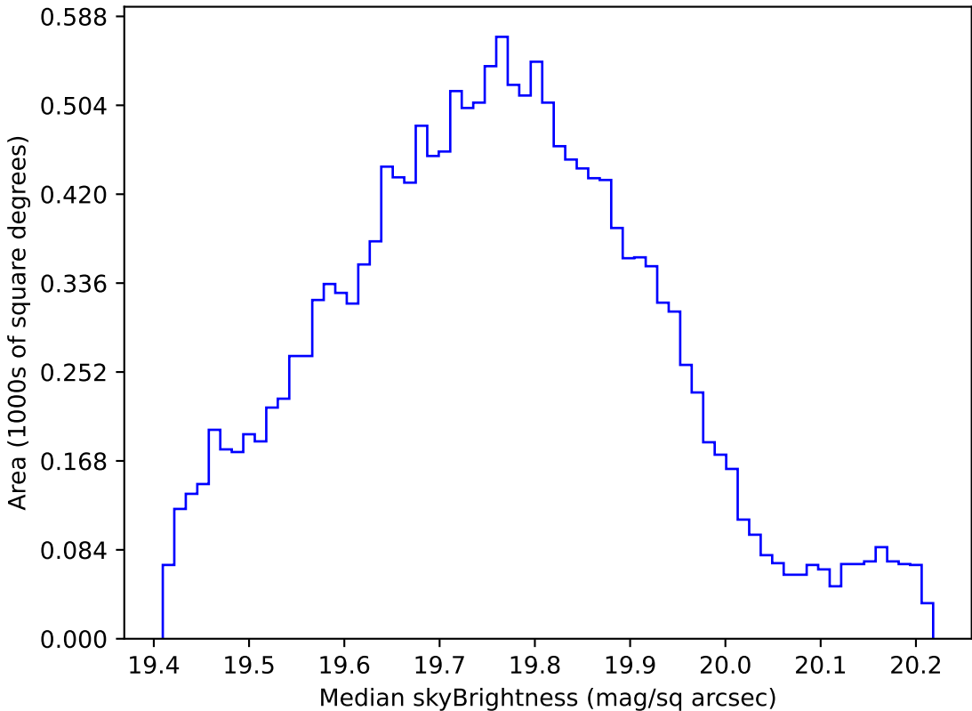
too_elab_r32_d2_griz_v3.4_10yrs WFD all bands: Median skyBrightness
