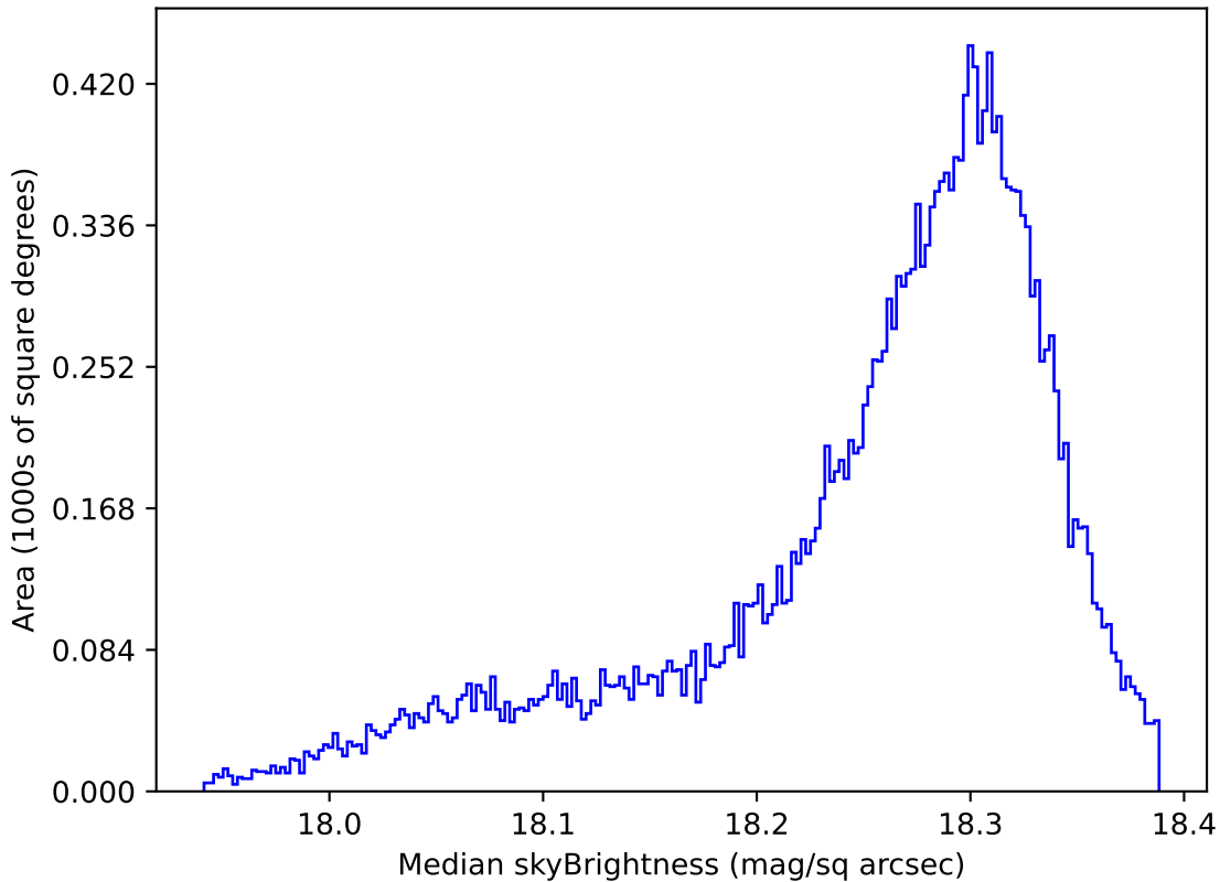
too_elab_r32_d2_griz_v3.4_10yrs All sky y band: Median skyBrightness
