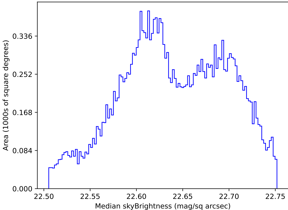
too_elab_r32_d2_griz_v3.4_10yrs All sky u band: Median skyBrightness
