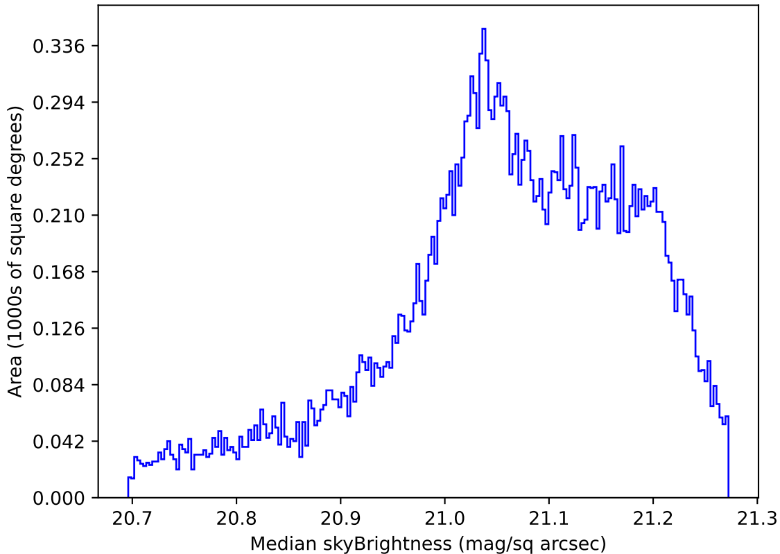
too_elab_r32_d2_griz_v3.4_10yrs All sky r band: Median skyBrightness
