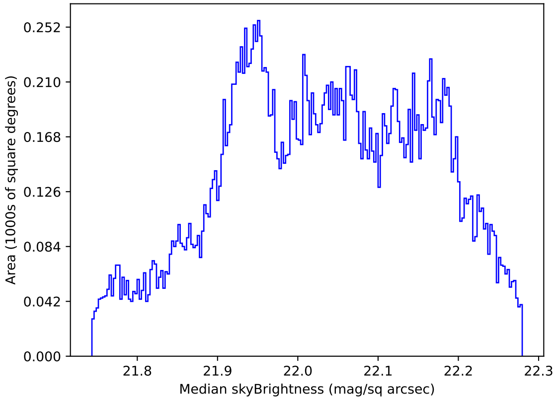
too_elab_r32_d2_griz_v3.4_10yrs All sky g band: Median skyBrightness
