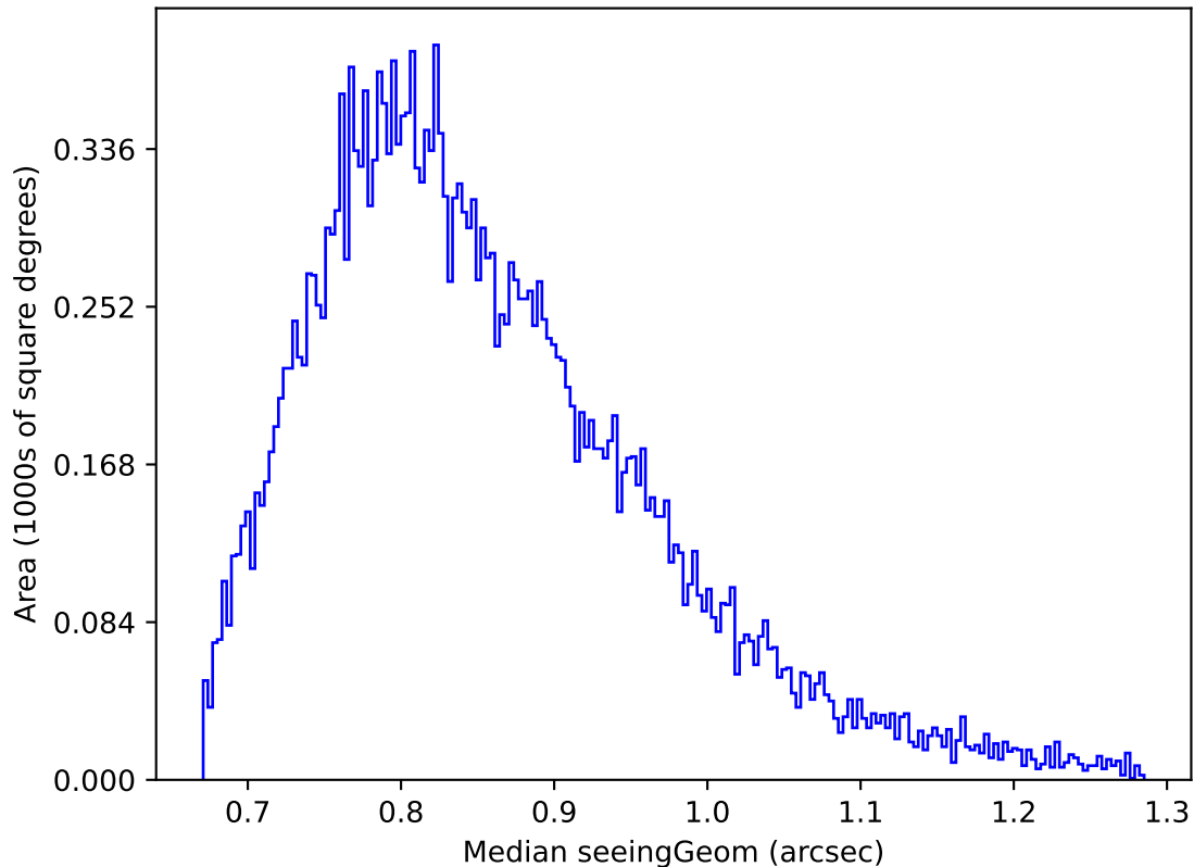
too_elab_r32_d2_griz_v3.4_10yrs Yr 1 z band: Median seeingGeom
