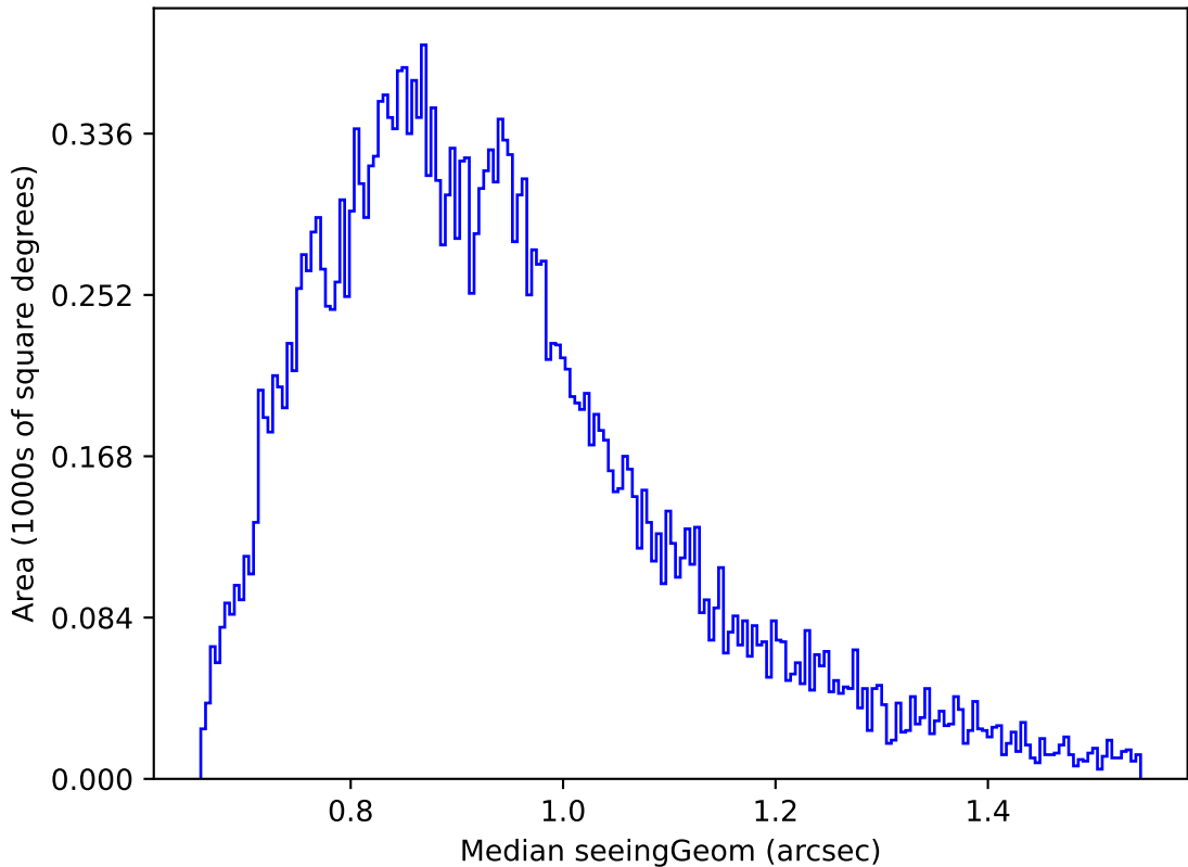
too_elab_r32_d2_griz_v3.4_10yrs Yr 1 g band: Median seeingGeom
