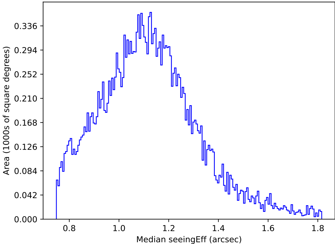
too_elab_r32_d2_griz_v3.4_10yrs Yr 1 u band: Median seeingEff
