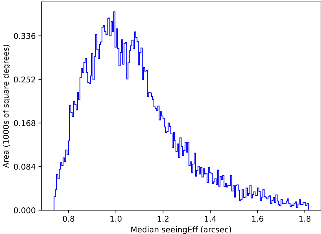
too_elab_r32_d2_griz_v3.4_10yrs Yr 1 g band: Median seeingEff
