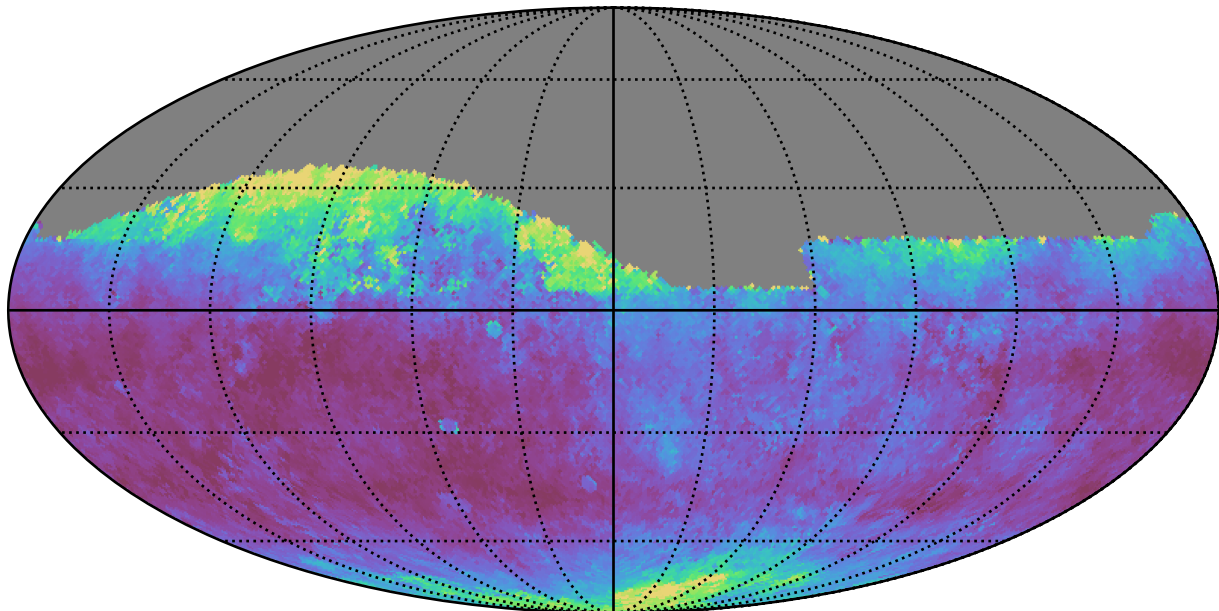
too_elab_r32_d2_griz_v3.4_10yrs Yr 1 all bands: Median seeingEff
