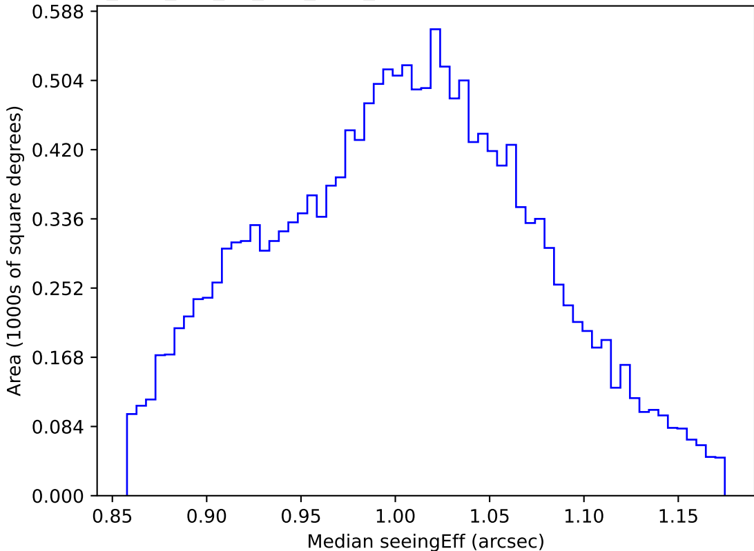
too_elab_r32_d2_griz_v3.4_10yrs WFD z band: Median seeingEff
