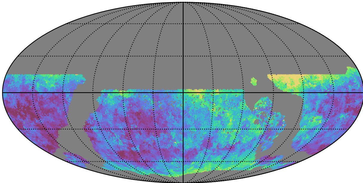
too_elab_r32_d2_griz_v3.4_10yrs WFD u band: Median seeingEff
