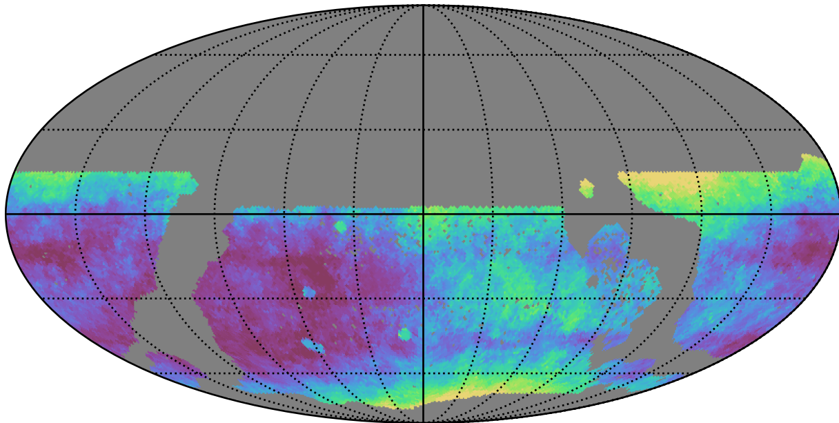
too_elab_r32_d2_griz_v3.4_10yrs WFD r band: Median seeingEff
