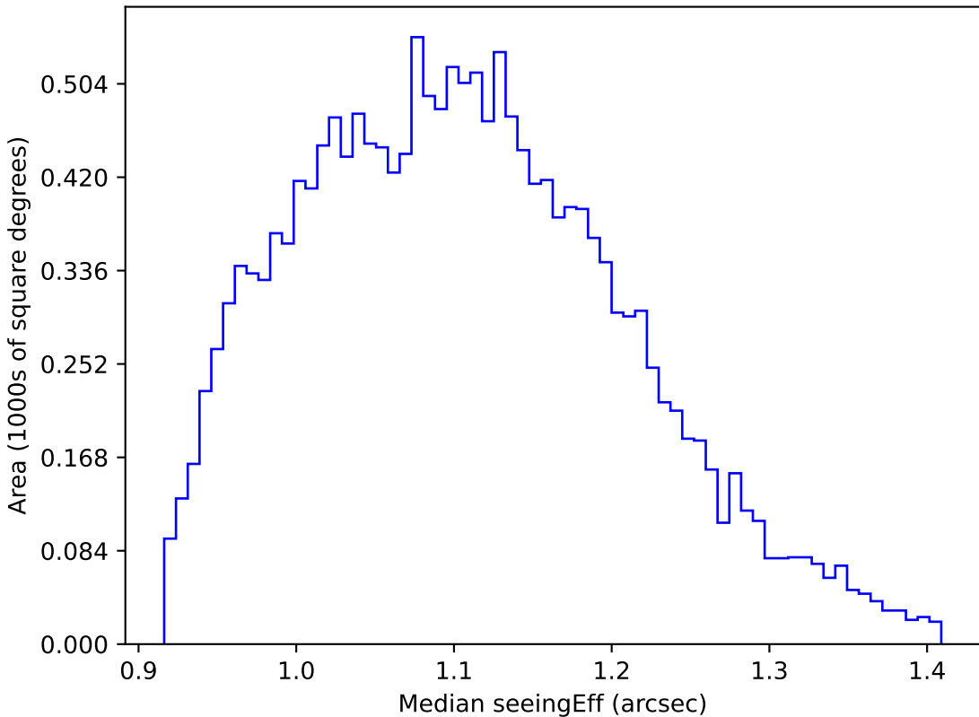
too_elab_r32_d2_griz_v3.4_10yrs WFD g band: Median seeingEff
