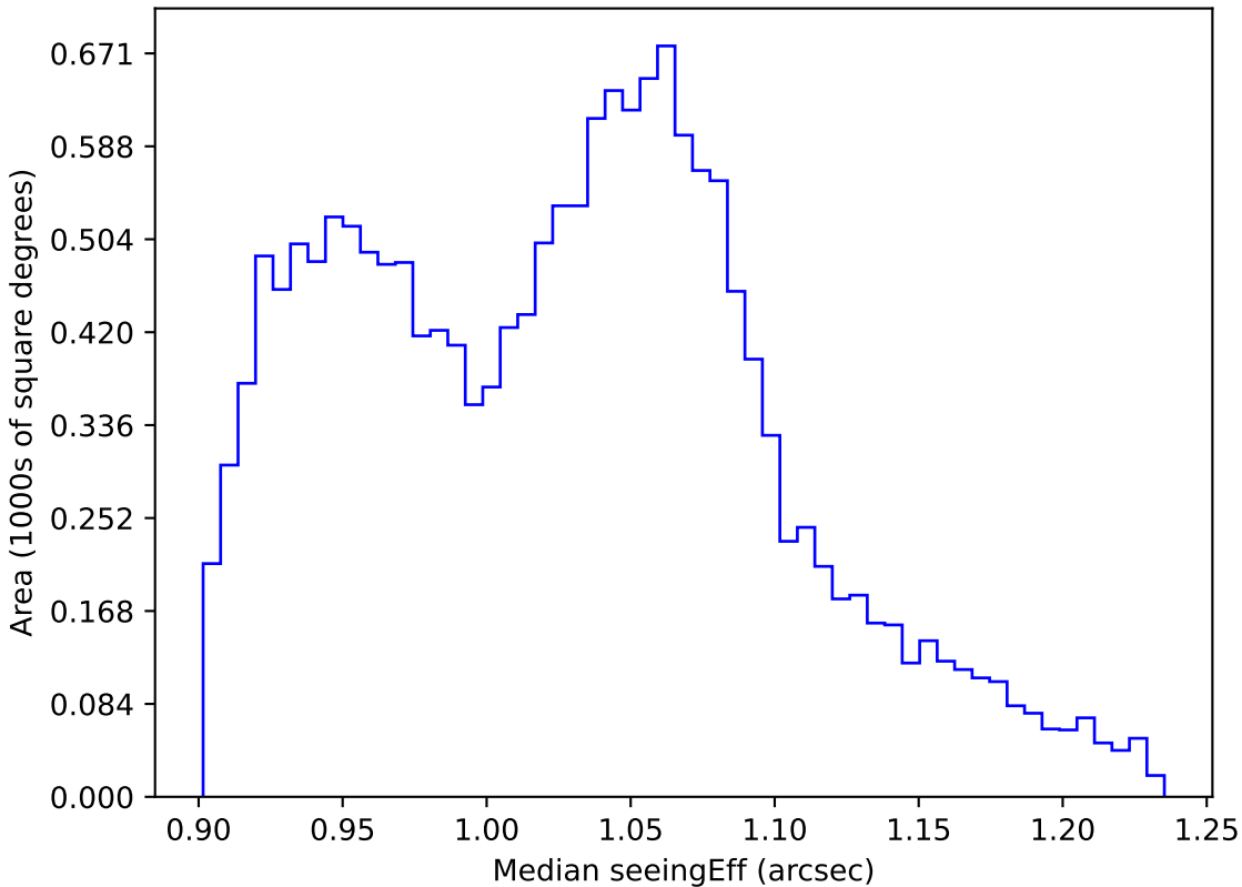
too_elab_r32_d2_griz_v3.4_10yrs WFD all bands: Median seeingEff
